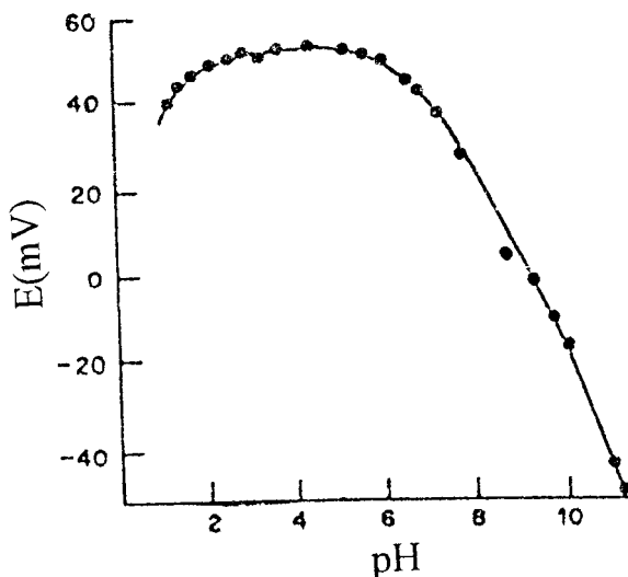
FIG. 2. Effect of pH on the potential of electrode c.
