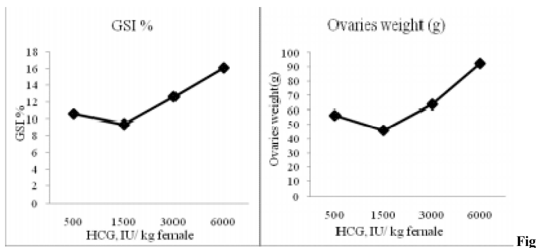
Fig 1. Changes of ovaries weight (g). Fig 2. Changes of gonadosomatic index
