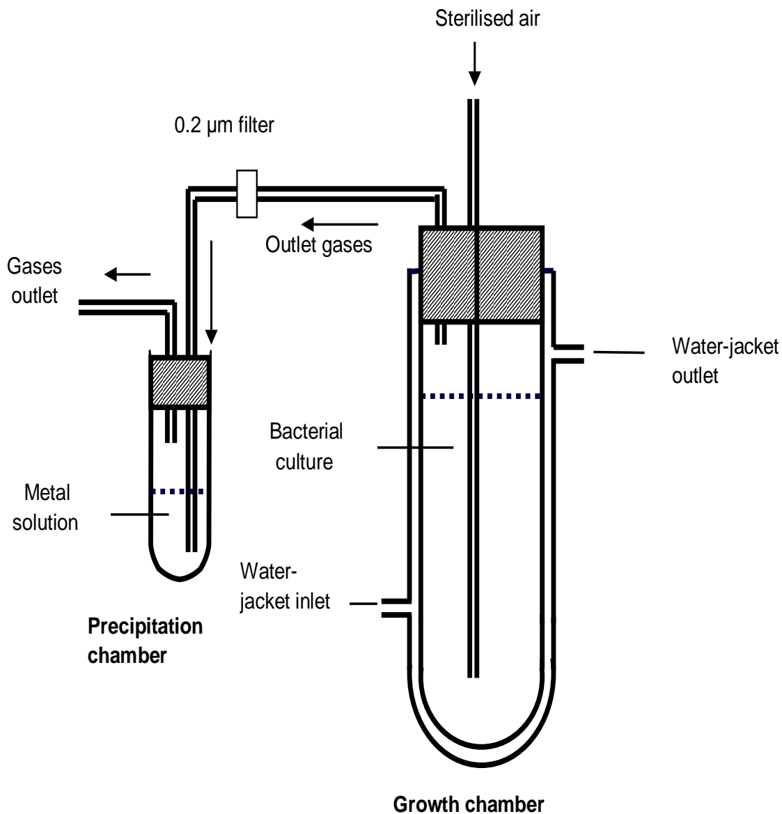
Figure 1. A bioreactor used for metal precipitation through the culture off-gas consisting of two chambers. The large vessel is the bacterial growth chamber and the second is the metal precipitation chamber. The growth vessel was held at 30°C through the water jacket and an external water bath.
