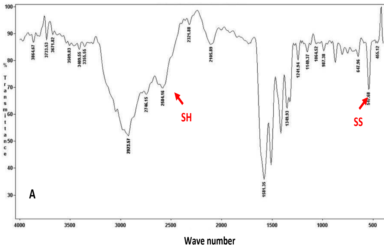
Figure 4. FTIR spectra of the single metal precipitates of (A) Mercury; (B) Cadmium and lead and; (C) Copper, zinc, nickel, cobalt, iron and manganese obtained using the culture biogases of the bacterial population of the activated sludge.
