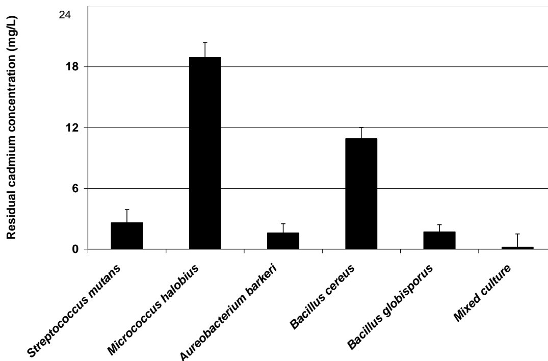
Figure 2. A comparison between the different bacterial isolates ( Micrococcus halobius , Streptococcus mutans , Aureobacterium barkeri , Bacillus cereus and Bacillus globisporus ) for cadmium bioremoval ( O.D_{600} = 1.3 \pm 0.8 ) after 24 h of exposure time. Initial concentration of cadmium was 32.3 mg/L. Data are the means of three replicates and error bars represent the standard errors of the means.
